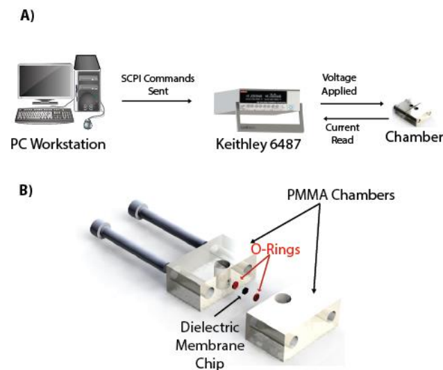
Figure 1. Schematic of Nanopore Experimental Setup. A) A Keithley 6487 Pico Ammeter/Voltage source applies a sustained high voltage electrical field across a dielectric membrane fastened in between our experimental chamber. The voltage source is controlled through a MATLAB script that is run through the PC workstation. As the voltage is being applied, the leakage current is measured simultaneously by the voltage source. B) Horizontal experimental chamber sandwiches a dielectric membrane in between two PMMA compartments tightened by screws. Two rubber O-rings are used to create an airtight seal. The openings in the O-rings create a nanotunnel that focuses the possible area of fabrication into a smaller region of the free-standing membrane.
